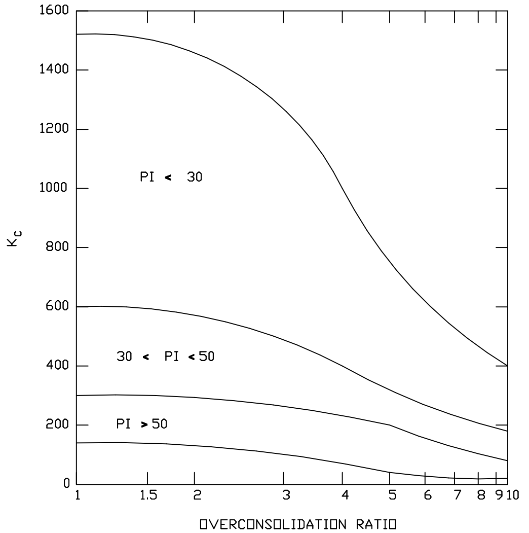
CHART FOR ESTIMATING CORRELATION FACTOR, K_c
